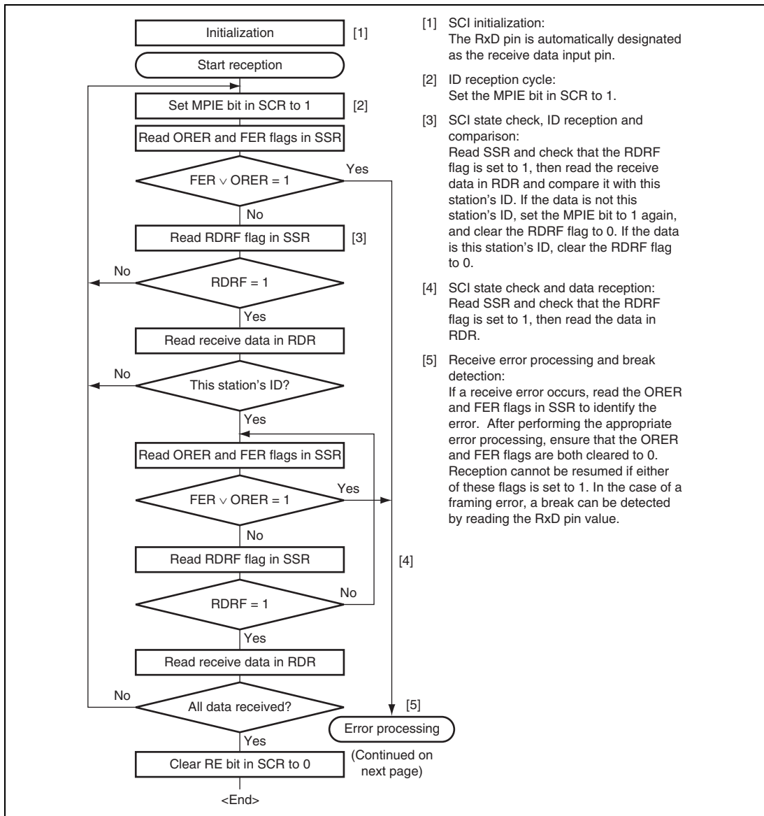
Figure 17.16 Sample Multiprocessor Serial Reception Flowchart (1)
