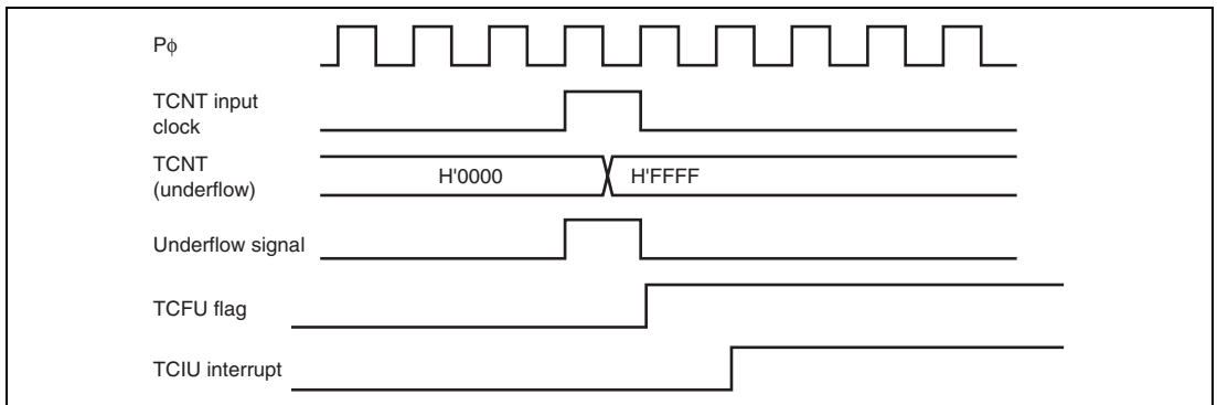
Figure 13.42 TCIU Interrupt Setting Timing
