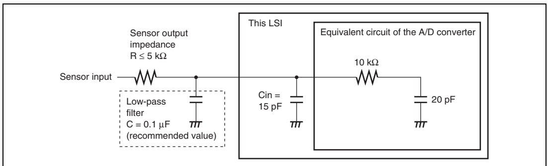
Figure 19.12 Example of Analog Input Circuit
