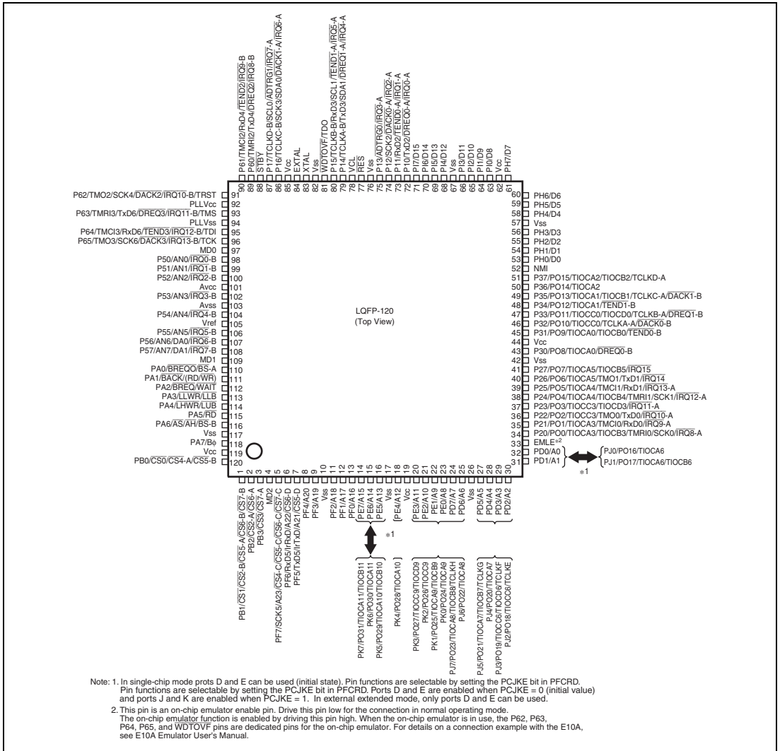
Figure 1.3 Pin Assignments
